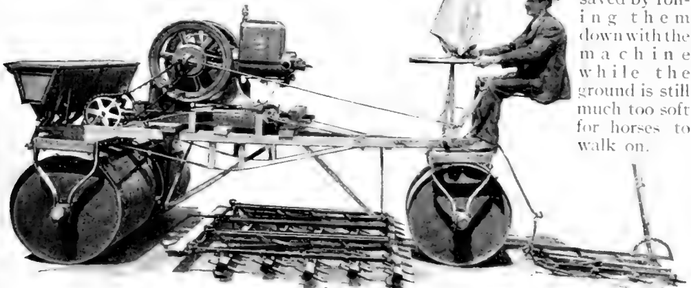
The Combined Roller and Harrow Which Does the Work of Four Horses and Two Men at a Cost of One and One Half Cents an Acre, to Say Nothing of the Time Saved
